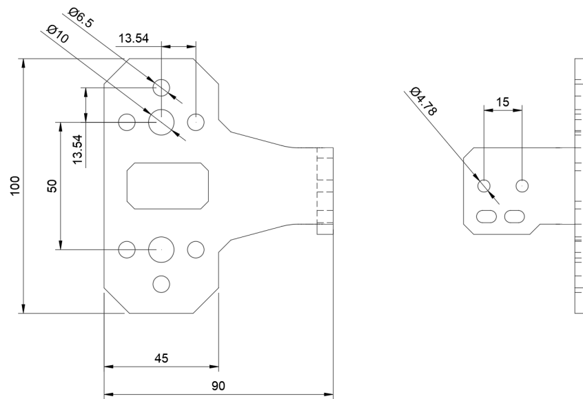
Fig. 4: Lower Mounting Part
