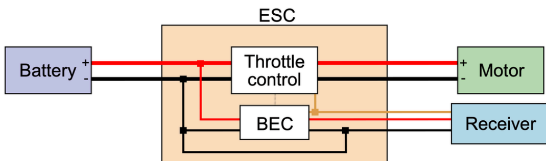
Figure 22: Drone power circuit including an ESC and a BEC
