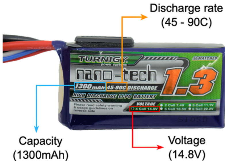
Figure 13: LiPo battery labels
