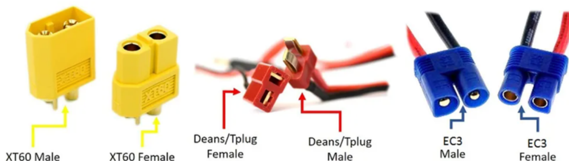
Figure 23: Common battery connectors, image from modelflight.com
